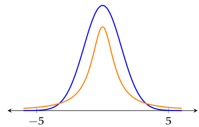
Figure 2.15: Standard normal distribution (blue) in comparison to the t-distribution with one degree of freedom ( \nu = 1 ) (orange). The t-distribution has more probability mass at the tails. Note that this demonstration shows a particularly exaggerated difference since \nu = 1 is the case with the largest difference between the t-distribution and the standard normal distribution. The difference diminishes with increased degrees of freedom.
