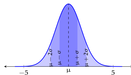
Figure 2.14: Normal PDF, with \mu = 0 and \sigma = 1 .
